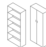
5 Tier Bookcase Includes 4x 22mm adjustable shelves Solid 22mm base with Adjustable ferruls 800 X 315 X 1860 Open, Assembled 711 104 008 Open, Knock Down 711 104 012 Doors, Assembled 711 105 005 Doors, Knock Down 711 105 009
