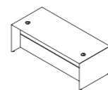
Platinum Executive Desk only 2000 x 900 x 732 32mm top, 22mm sides 721 210 005
