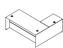
Platinum Executive Desk with extension (LHS) 2000 x 1800 x 732 32mm top, 22mm sides 721 210 001
